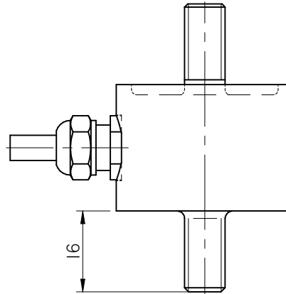
STUD BASE COMPRESSION: ORDER CODE 'D' TENSION: ORDER CODE 'T' BI-DIRECTIONAL: ORDER CODE 'U'
