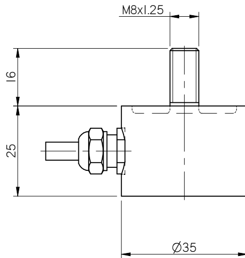
FLAT BASE COMPRESSION: ORDER CODE 'C'
