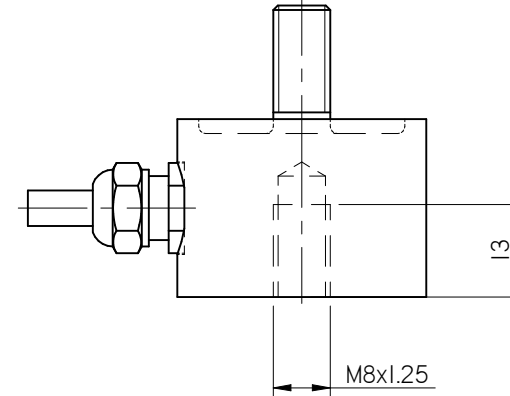
FEMALE BASE COMPRESSION: ORDER CODE 'A' TENSION: ORDER CODE 'G' BI-DIRECTIONAL: ORDER CODE 'J'
