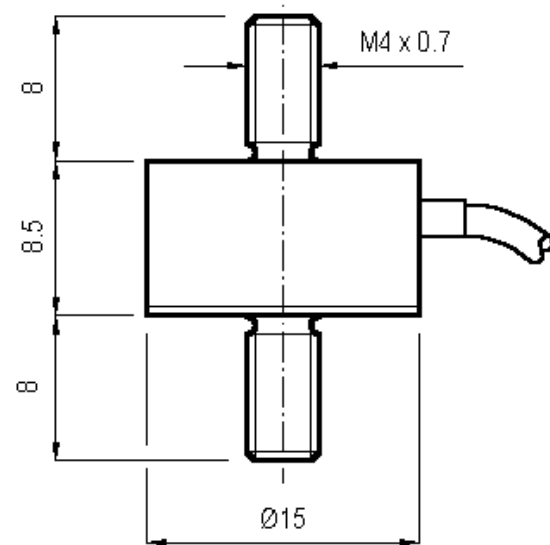
STUD VERSION TENSION AND/OR COMPRESSION
